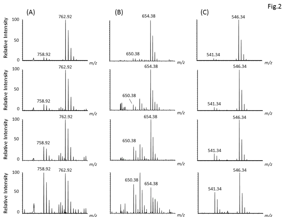
Figure 2: Representative mass spectra of spiked-in labeled standard peptides and corresponding unlabeled endogenous peptide using post-digestion spike-in approach. (A) Mass spectra of labeled and unlabeled peptide pairs detected after spiking in-gel digested dystrophin with varying amounts of ^{13}\text{C}_6 , ^{15}\text{N}_2 Lysine labeled standard peptide [IFLTEQPLEGLEK]. (B) Shows mass spectra of labeled and unlabeled peptide pairs detected after spiking in-gel digested dystrophin with varying amounts of ^{13}\text{C}_6 , ^{15}\text{N}_2 Lysine labeled standard peptide [LLDLLLEGLTGQK]. (C) Shows mass spectra of labeled and unlabeled peptide pairs detected after spiking in-gel digested dystrophin with varying amounts of ^{13}\text{C}_6 , ^{15}\text{N}_4 Lysine labeled standard [LLVEELPLR]. The concentration of each spike-in standard peptide, starting for the top to the low panels, was as follows (160 nM, 80 nM, 40 nM and 14 nM). Samples were analyzed on the LTQ-Orbitrap XL at 30,000 resolution and mass error better than 10 ppm. All ions were detected as doubly protonated species with the correct m/z values.
