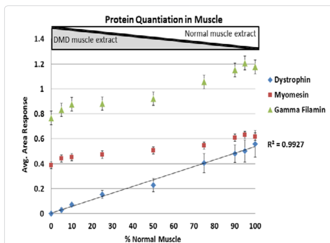
Figure 5: Titration curve of dystrophin protein and other muscle specific proteins using pre-digestion spike-in approach. Dystrophin protein, as well as myomesin and filamin c, were quantitated in different combination mixtures of muscle extracts from DMD and age matched healthy donors at ratios leading to 0, 5, 10, 25, 50, 75, 90, 95 and 100% of dystrophin relative to normal. Each final mixture contained 50 µg of total muscle protein and was spiked with 25 µg of ^{13}\text{C}_6 -Lysine labeled SILAC mouse muscle extract. Gel bands encompassing dystrophin protein and other muscle specific proteins were excised and processed for mass spectrometry analysis as described in Methods. Transition ion intensities obtained at the MS/MS level for the targeted labeled and unlabeled peptide pairs generated from the spike-in standard and endogenous human dystrophin were used to determine the relative amount of dystrophin and other muscle proteins (myomesin and filamin c). Standard deviation at each data point represents average ratios obtained from labeled and unlabeled peptide pairs: 5 pairs for dystrophin protein (QAPIGGDFPAVQK, VLSQIDVAQK, IFLTEQPLEGLEK, TLNATGEEIIQQSSK, VHALLNNVKNK); 3 pairs for filamin c (SPFVVNVAPPLDLSK, EVGEHVVSVRK, HIGISFTPK) and two pairs for myomesin (VSEPVAALDPAEK, VLGGLPDW-TIQEGK). These peptides have 100% sequence homology between human and mouse and were used for ratio measurements. As expected, dystrophin protein increased with increasing relative amount of normal muscle extract while myomesin and filamin c remained unchanged.
