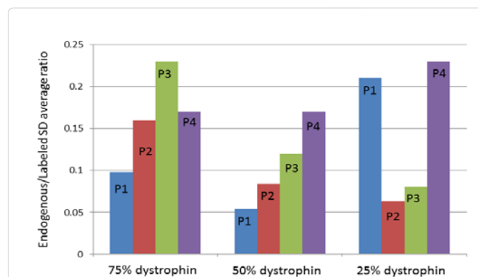
Figure 4: Inter sample reproducibility of the post-digestion spike-in approach. Three samples containing varying amount of dystrophin obtained by mixing muscle extract from a DMD and age matched healthy donor at ratio of 25/75, 50/50 and 75/25 respectively were evaluated for dystrophin quantitation using the post-digestion spike-in approach with 30 nM of stable isotope standard peptides. Histograms represent intensity ratios of endogenous dystrophin peptides and filamin c peptide to their corresponding stable isotope labeled standard peptide. P1, P2 and P3 corresponds to dystrophin peptides [LLDLEGLTGQK], [LLVEELPLR], [IFLTEQPLEGLEK] respectively and P4 correspond to filamin c peptide [VYNVTYTVK] that was used as an internal control. It is clearly seen that some ratios did not decrease with decreasing amounts of dystrophin, especially for the peptide P1, showing high variability for this approach.
